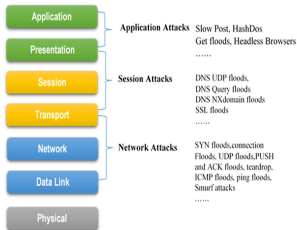
Figure 2. The layering of DDoS attacks on the OSI network model
