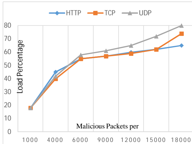
Figure 5. CPU Load Results
