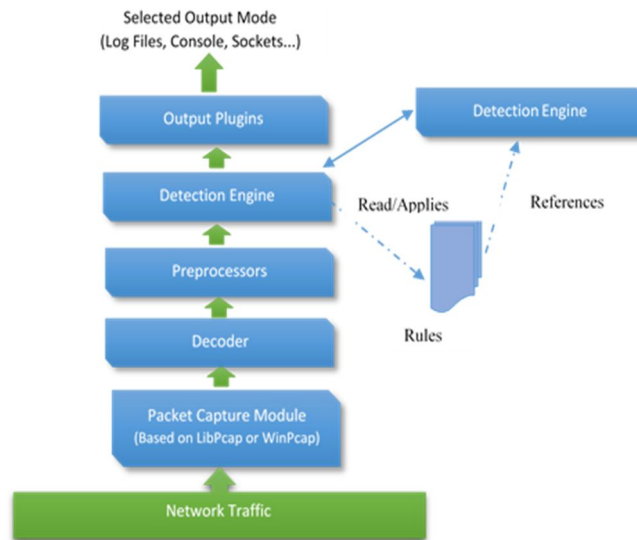
Figure 3. Architecture of Snort
