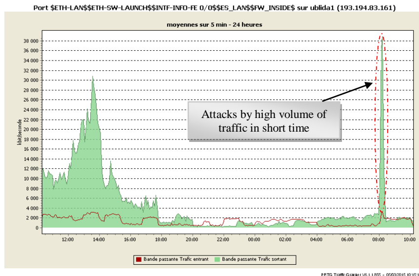
Figure 6. Campus network traffic under attack.
