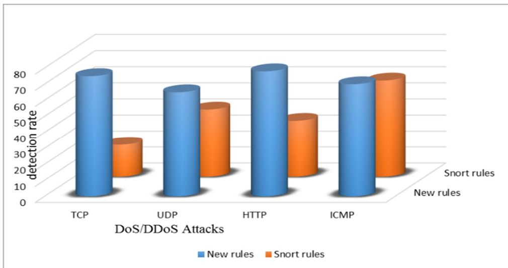
Figure 6. Comparison between Snort rules and new ones
